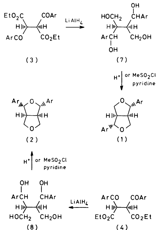
SCHEME 3
